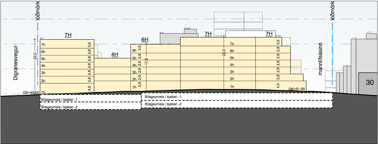
SNID A-A, mkv 1:500 (A3)
