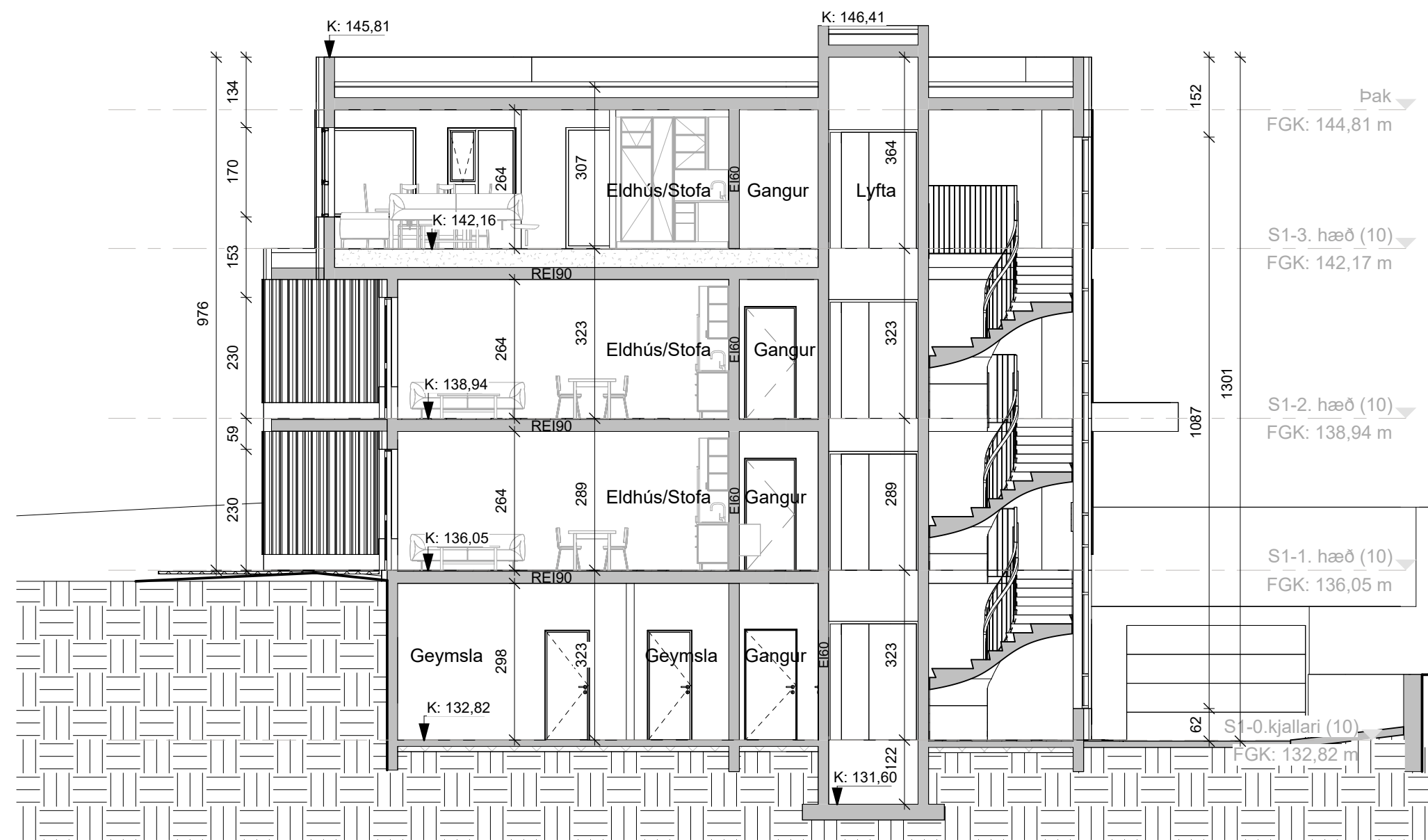
D-1 Sneiðing D (S1) 1 : 100
