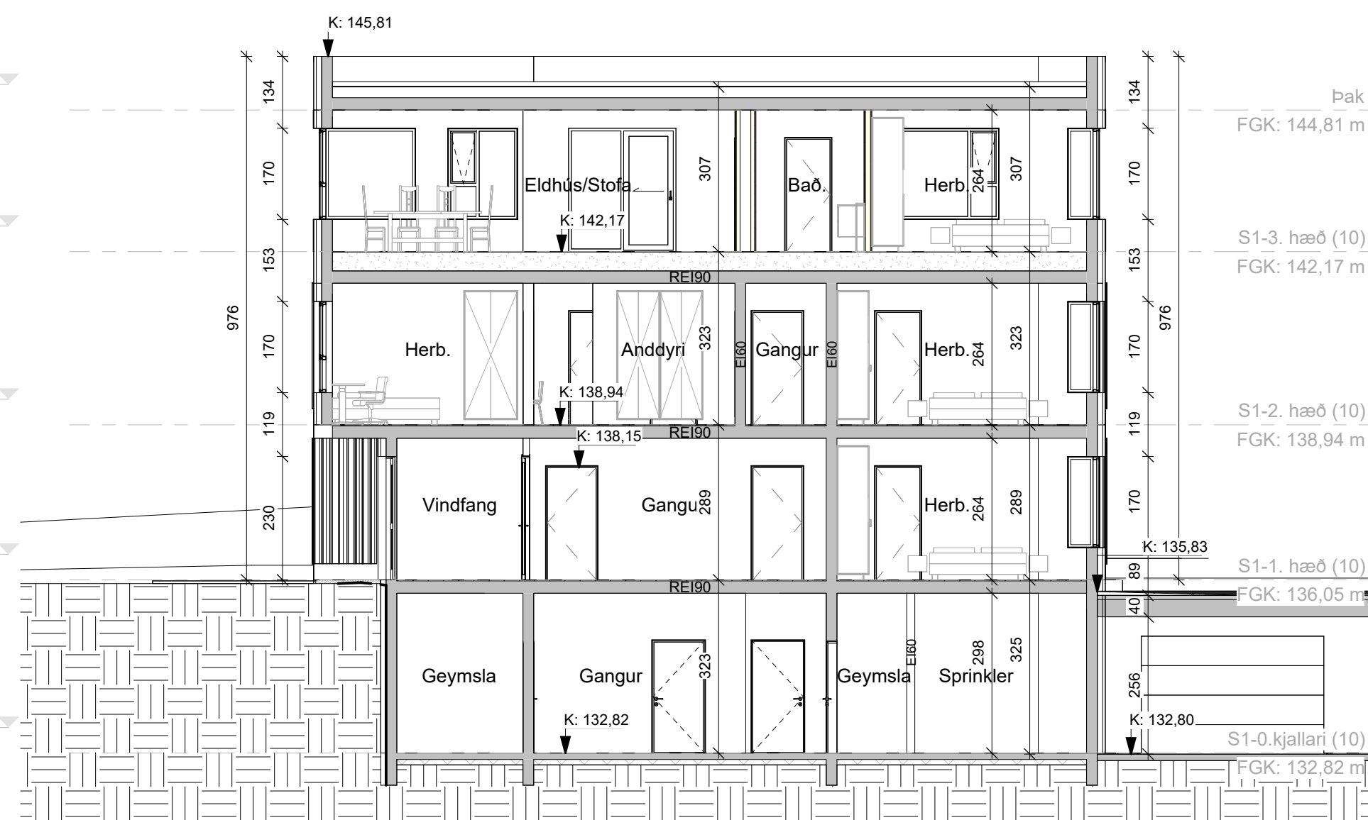
C-1 Sneiðing C (S1) 1 : 100
