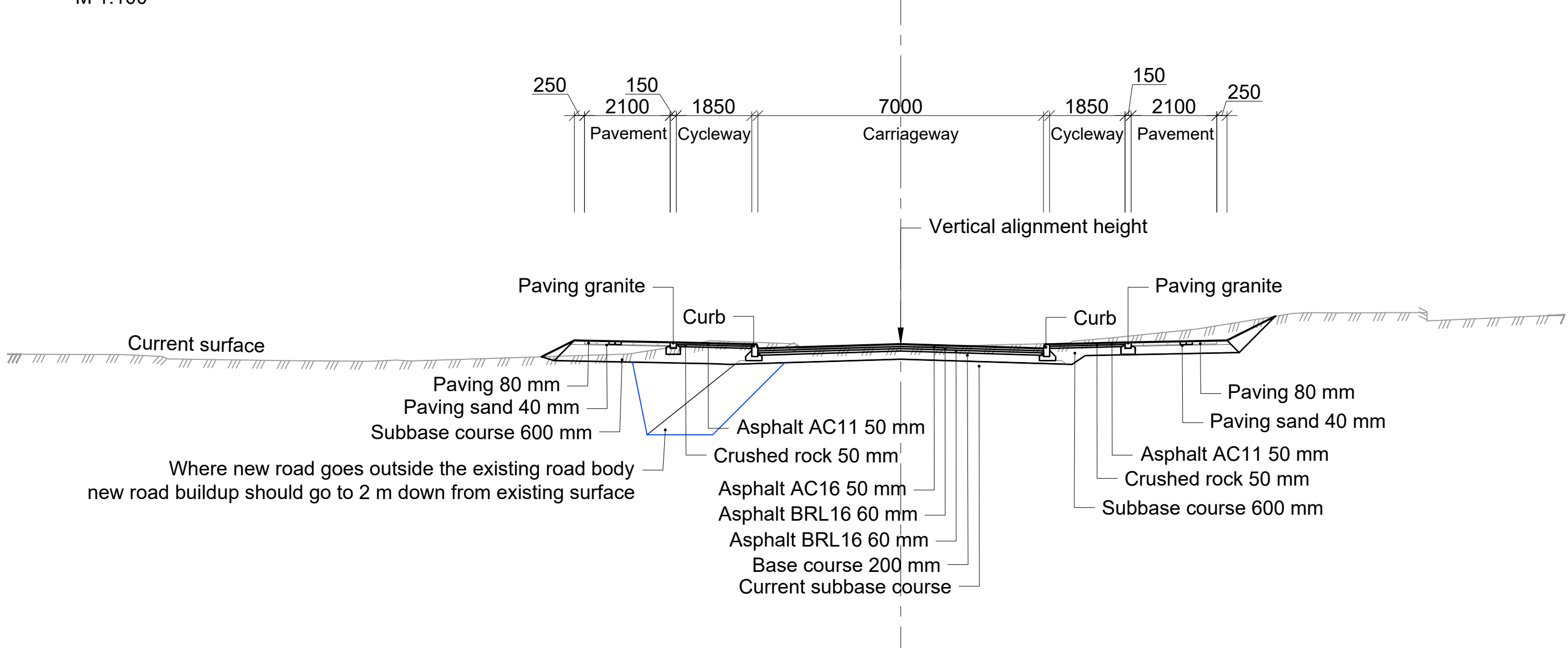
Borgarlínan - Characteristic section St. approx. 9700 M 1:100
