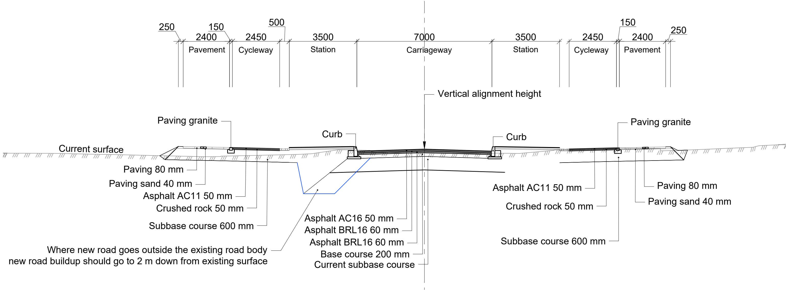
Borgarlínan - Characteristic section St. approx. 9770 M 1:100
