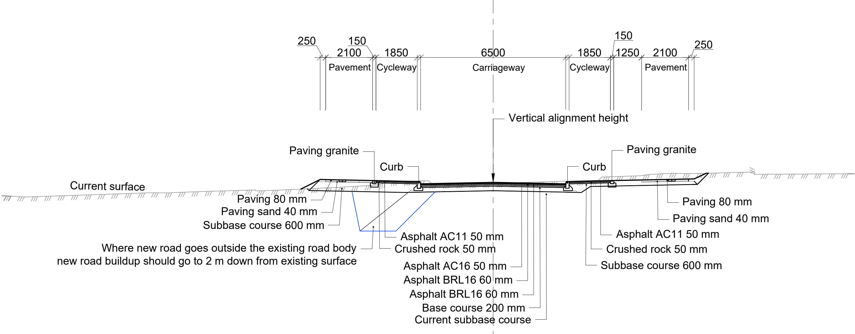
Borgarlínan - Characteristic section St. approx. 9630 M 1:100
