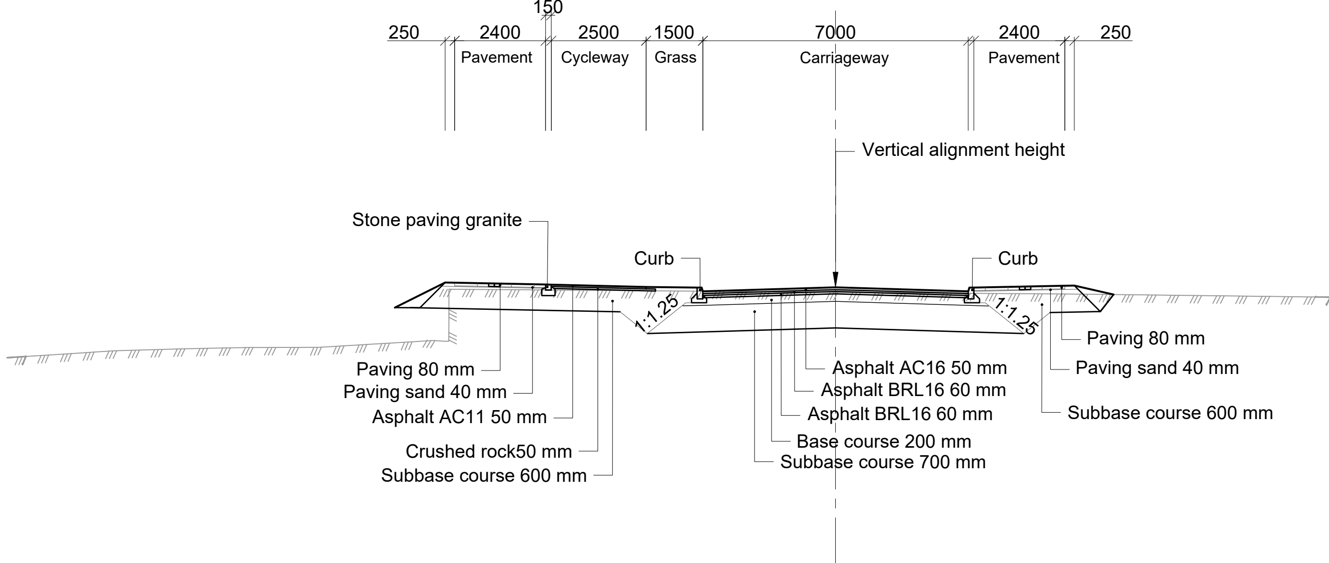
Borgarlínan - Characteristic section St. approx. 9900 M 1:100
