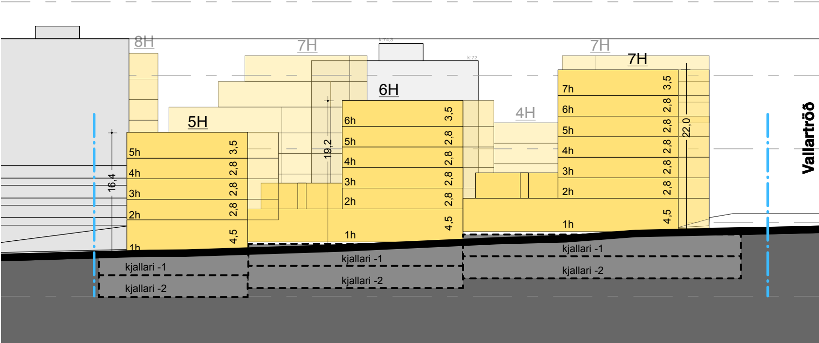
SNID C-C, mkv 1:500 (A3)
