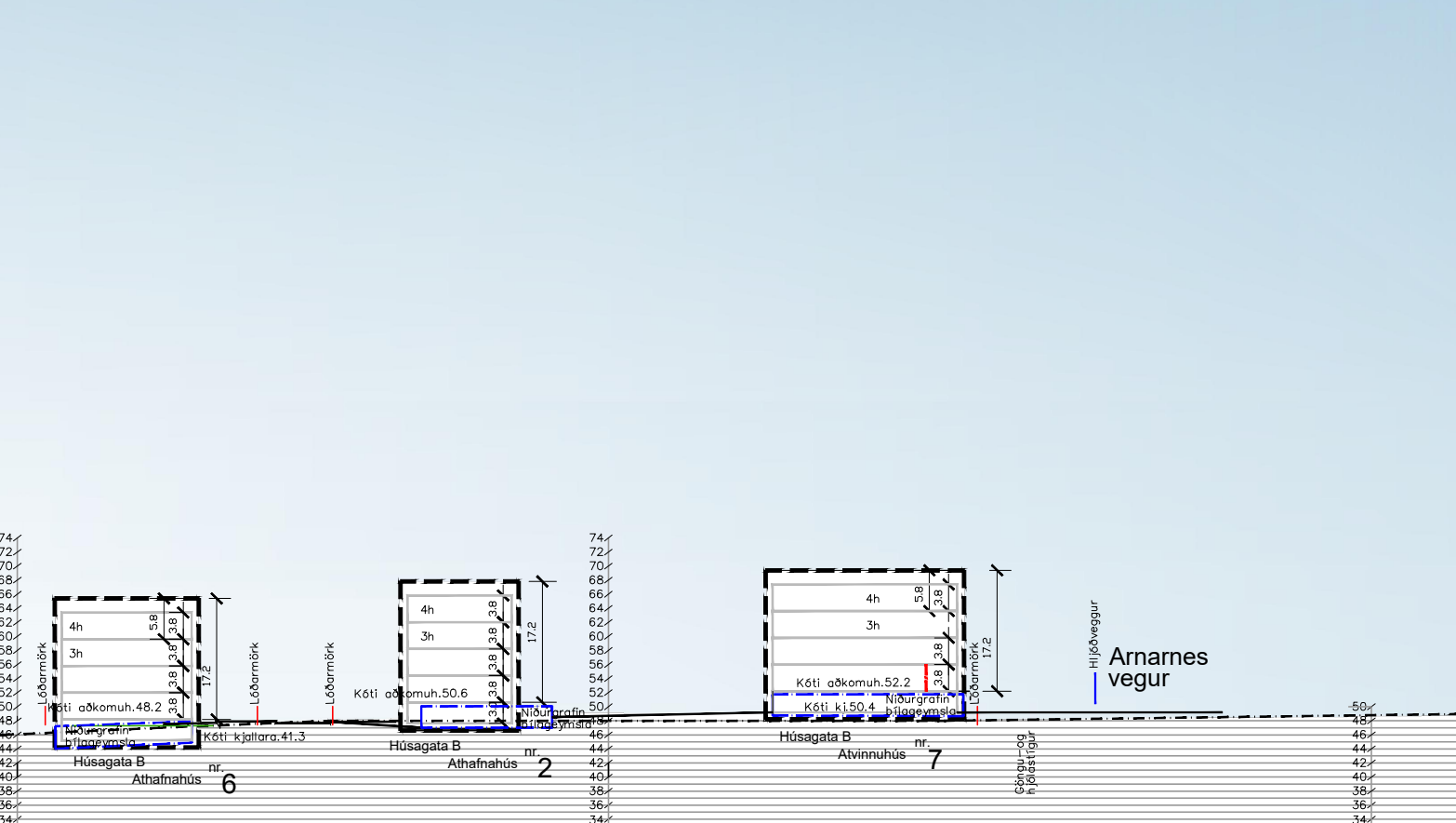
Shedding B - B I mkv. 1:1000
